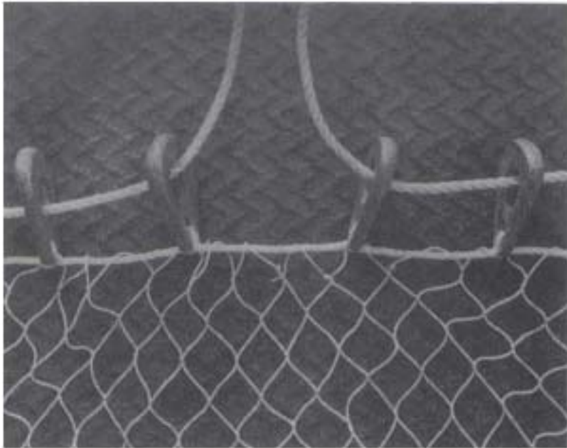
Leadline with rings and purse line
