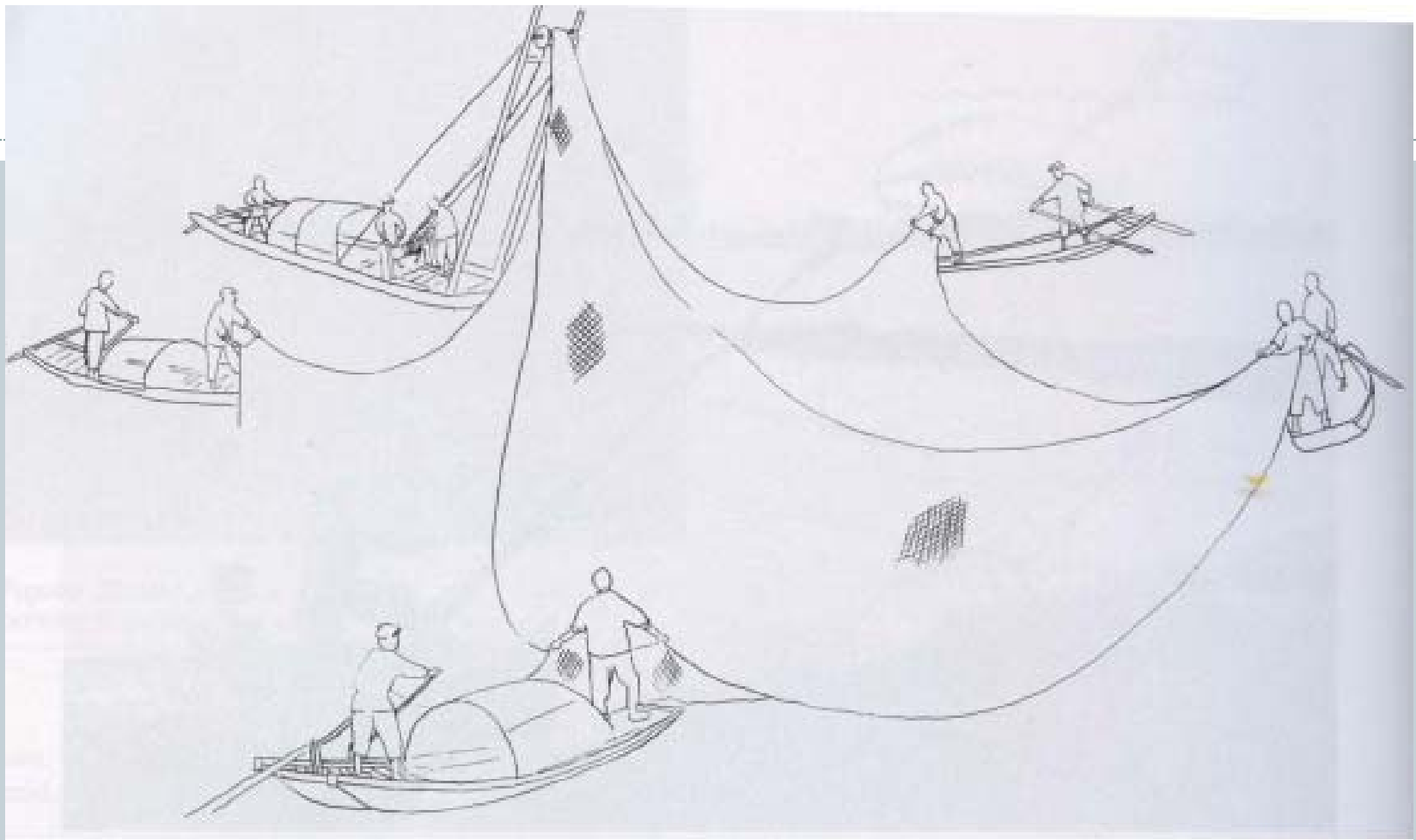
Newer Chinese giant-size cast net for a fresh water fishery operated from a net boat with winch and four rowing boat
